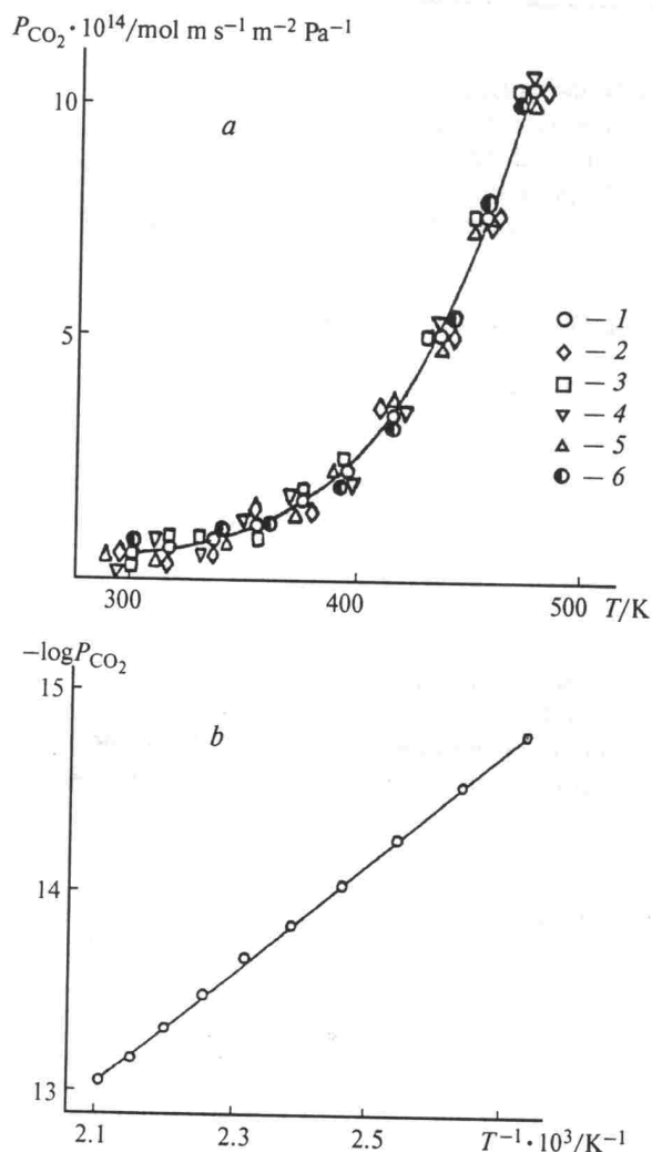
Fig. 3. Temperature influence ( T ) on the permeability coefficients of \text{CO}_2 ( P_{\text{CO}_2} ) through perfluorosulfonic membranes in the \text{Cr}^{3+} (1), \text{Fe}^{3+} (2), \text{Co}^{2+} (3), \text{Ni}^{2+} (4), \text{Cu}^{2+} (5), and \text{Zn}^{2+} (6) ionic forms in the coordinates P_{\text{CO}_2}-T (a) and (-\log P_{\text{CO}_2})-(T^{-1}) (b).
