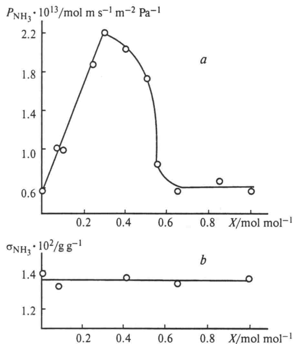
Fig. 5. Permeability coefficient of NH 3 (P NH 3 ) (a) and coefficient of its solubility σ (b) for the perfluorosulfonic membranes in the mixed Cu 2+ -Zn 2+ form as functions of the molar fraction of Cu 2+ (X) in the membrane at T = 295 K (p H 2 O = 0).
