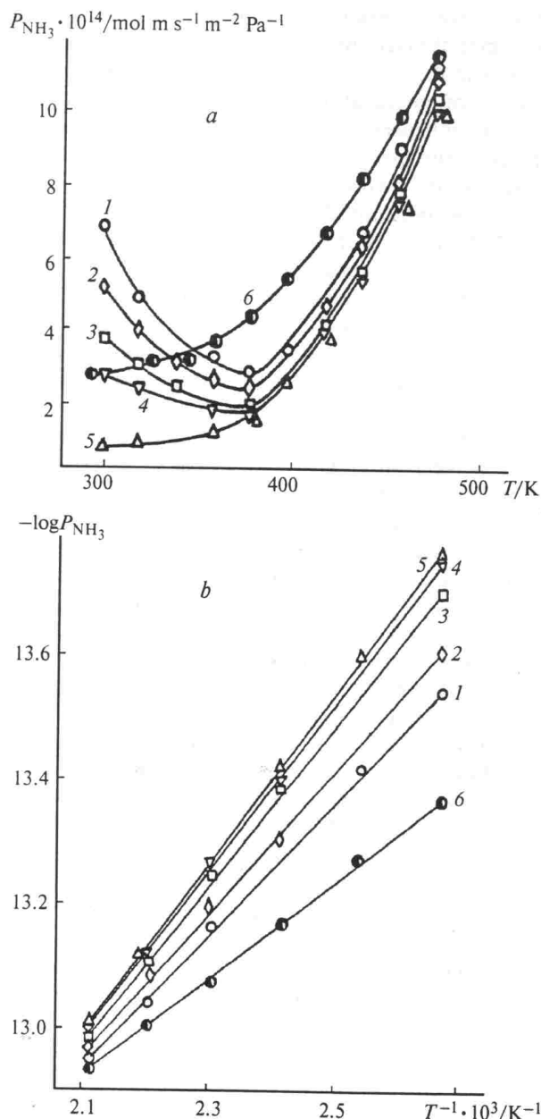
Fig. 2. Temperature influence ( T ) on the permeability coefficients of \text{NH}_3 ( P_{\text{NH}_3} ) through perfluorosulfonic membranes in the \text{Cr}^{3+} (1), \text{Fe}^{3+} (2), \text{Co}^{2+} (3), \text{Ni}^{2+} (4), \text{Cu}^{2+} (5), and \text{Zn}^{2+} (6) ionic forms in the coordinates P_{\text{NH}_3} – T (a) and (-\log P_{\text{NH}_3}) – (T^{-1}) (b).
