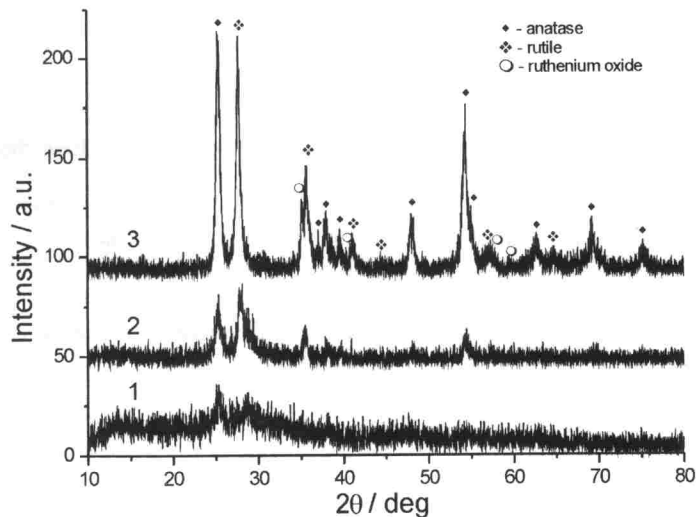
Fig. 4 XRD patterns of (\text{TiO}_2)_{0.9}(\text{RuO}_2)_{0.1} \cdot 1.5\text{H}_2\text{O} heated in argon 1 – initial sample, 2 – sample heated to 400^\circ\text{C} and 3 – to 600^\circ\text{C}
